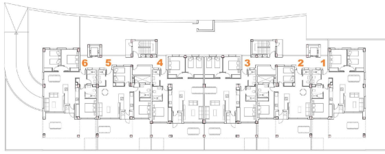
Planta Baja Ground Floor 0
